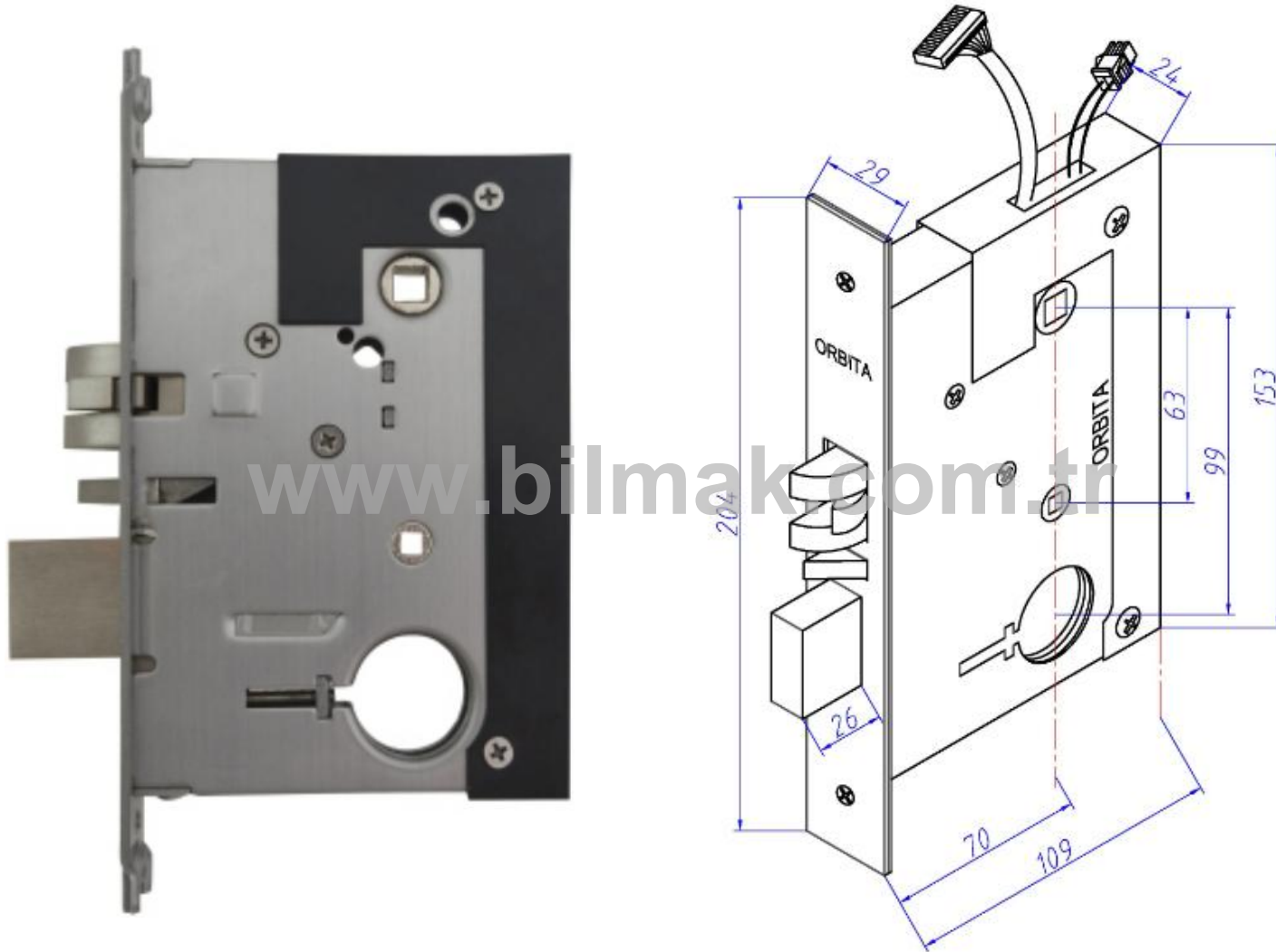
ANSI mortise, five latch, with deadbolt
